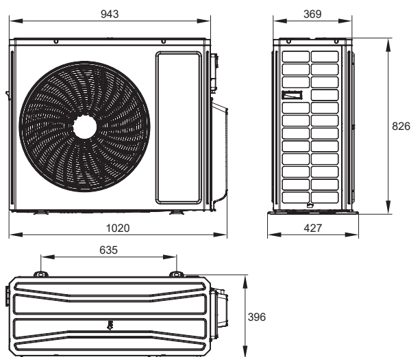
■ GWHD(36)NK600(LC)(LH) - GWHD(42)NK600(LC)(LH)
