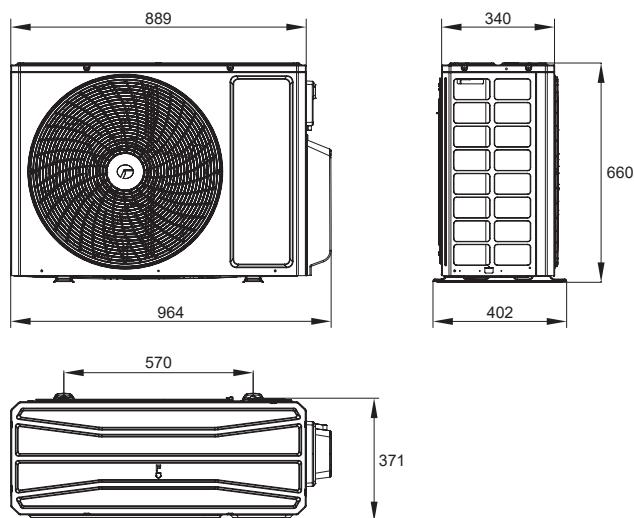
■ GWHD(24)NK600(LC)(LH) - GWHD(28)NK600(LC)(LH)
